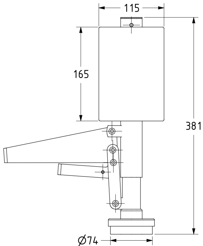
EXTENDED
