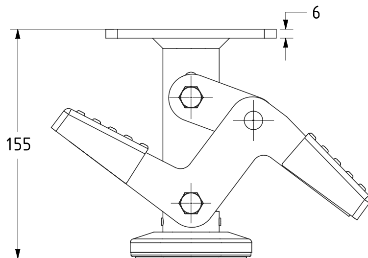
RETRACTED
