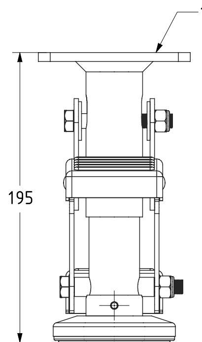
EXTENDED
